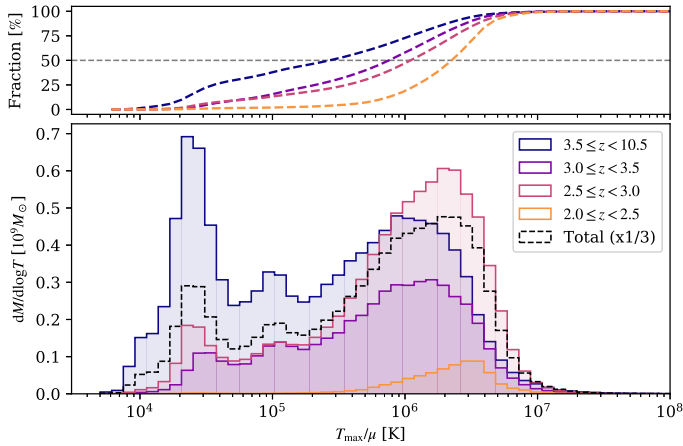
Fig. 16. Bottom panel: histogram of the maximum temperature of the gas accreted onto the central galaxy between different redshifts (from early accretion time in blue to late accretion time in yellow). Top panel: cumulative distribution of the gas temperature. Only the gas-forming stars within the virial radius are selected. The total distribution integrated over the total accretion time is shown with the black dashed line in the bottom panel. The total distribution has been rescaled by a factor of one third for visualisation. The halo has two modes of accretion: a cold and a hot mode. At high z the cold mode dominates and at low z the hot mode dominates.
