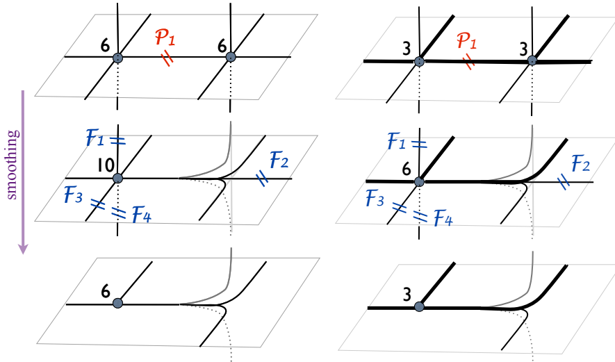
Figure 4.5.4: Following the cartoon shown in figure 4.5.3, the left panel shows a smoothing sequence (from top to bottom) which would preserve the connectivity of a 3D peak. It requires that each \mathcal{P} merger should be followed by four \mathcal{F} mergers in the vicinity. The right panel highlights how the multiplicity is preserved if one starts with 3 dominant co-planar filaments.
