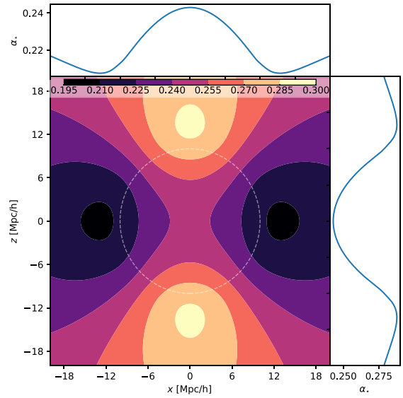
Figure C1. Isocontours in the x-z plane of the typical accretion rate \alpha_* around a wall-type saddle point [at (0, 0) ]. The saddle point is defined using the values of Table D1. The profiles in the main direction of the wall ( z -direction) and of the void ( x -direction) are plotted on the sides. The smoothing scale is R = 1 \text{ Mpc } h^{-1} . The typical accretion rate is computed using a \Lambda CDM power spectrum. Similarly to what happens in filaments, haloes accrete more in the direction of the wall than in the direction of the void.
